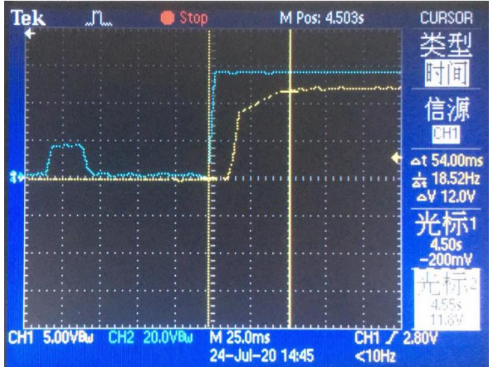
Output response &amp; load (12V / 0.01A)
