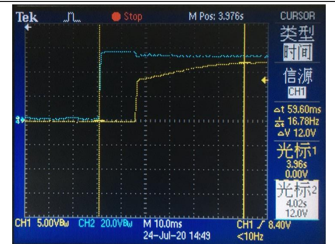
Output response &amp; load (12V / 1.1A)
